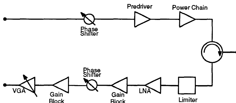
Figure 1: Block Diagram: Separate Transmit and Receive Module
